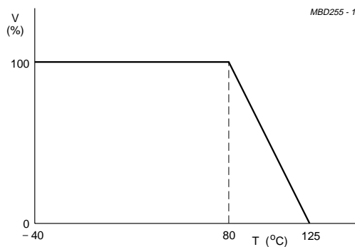
Fig.12 Derating curve.
