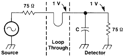
c). Calibration of Waveform Monitor Using Zero Ohm Characterization
