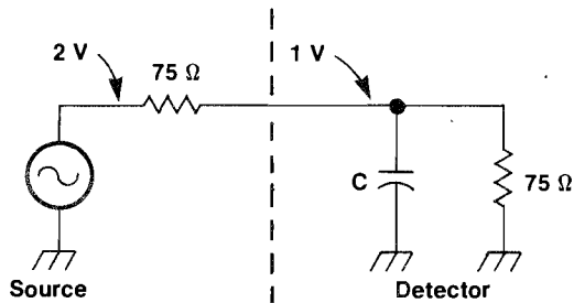
d). Calibration of Generator Using 75 Ohm Characterization
