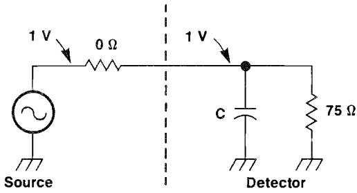
a). Detector Characterization from Zero Ohm Source
